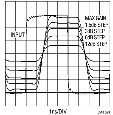
Pulse Response vs Attenuation, Output Level is 2\text{V}_{P-P} at Max Gain into 50\Omega External Load
