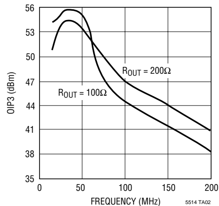
Output IP3 vs Frequency (Standard Mode)
